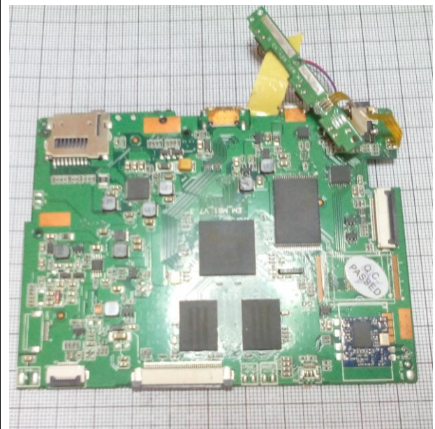
A1021 (SPPCBTERRA101)
